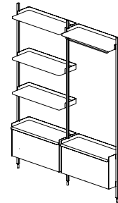
PIER SYSTEM | 1082 WIDTH 162 CM | 63.75" DEPTH 34 CM | 13.5" HEIGHT 209 CM | 82.25"
