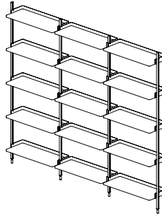
PIER SYSTEM | 113 WIDTH 242 CM | 95.25" DEPTH 31,5 CM | 12.50" HEIGHT 209 CM | 82.25"
