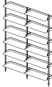
PIER SYSTEM | 102 WIDTH 162 CM | 63.75" DEPTH 31,5 CM | 12.50" HEIGHT 209 CM | 82.25"
