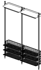
PIER SYSTEM | 1022 WIDTH 162 CM | 63.75" DEPTH 31,5 CM | 12.50" HEIGHT 209 CM | 82.25"
