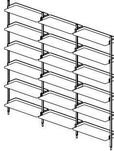
PIER SYSTEM | 103 WIDTH 242 CM | 95.25" DEPTH 31,5 CM | 12.50" HEIGHT 209 CM | 82.25"
