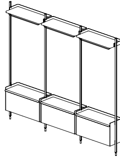
PIER SYSTEM | 1003 WIDTH 242 CM | 95.25" DEPTH 34 CM | 13.5" HEIGHT 209 CM | 82.25"
