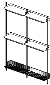
PIER SYSTEM | 1032 WIDTH 162 CM | 63.75" DEPTH 31,5 CM | 12.50" HEIGHT 209 CM | 82.25"
